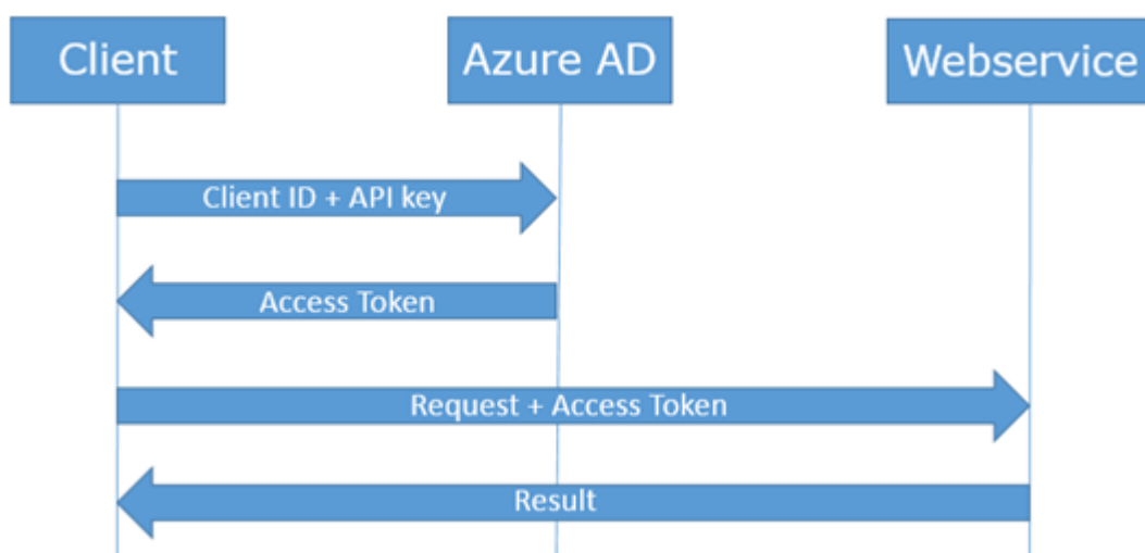
Figuur 1: Authentication flow
